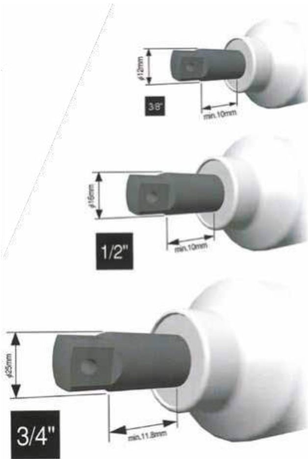
Sleeve Drive Sockets
