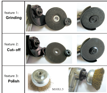
Assembled Instruction
