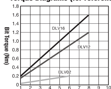
Torque Diagrams (for reference)
