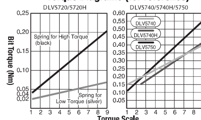
Torque Diagrams (for reference)
